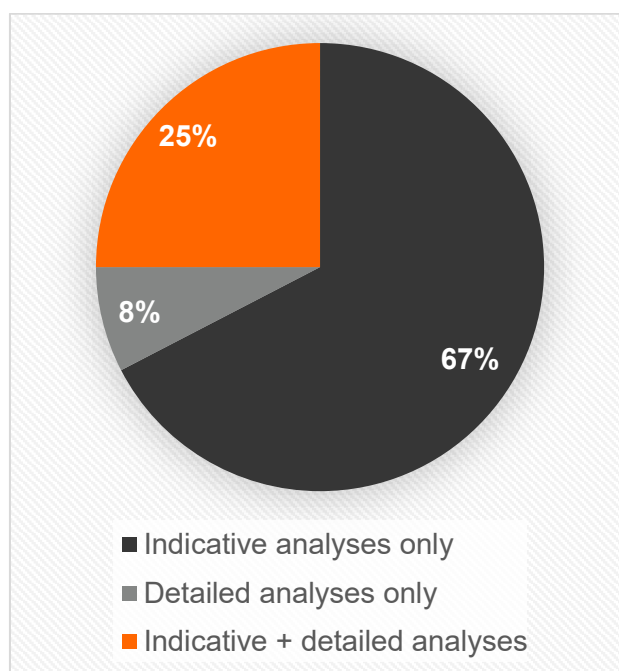
Figure 7. Analysis approaches.
