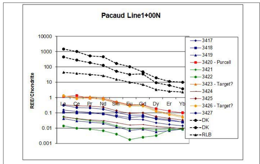
Figure 4: REE/Chondrite Plot for the Pacaud MMI™ Data. DK is the Field for Diamondiferous Kimberlites. RLB is the Round Lake Batholith from Berger (2006)
