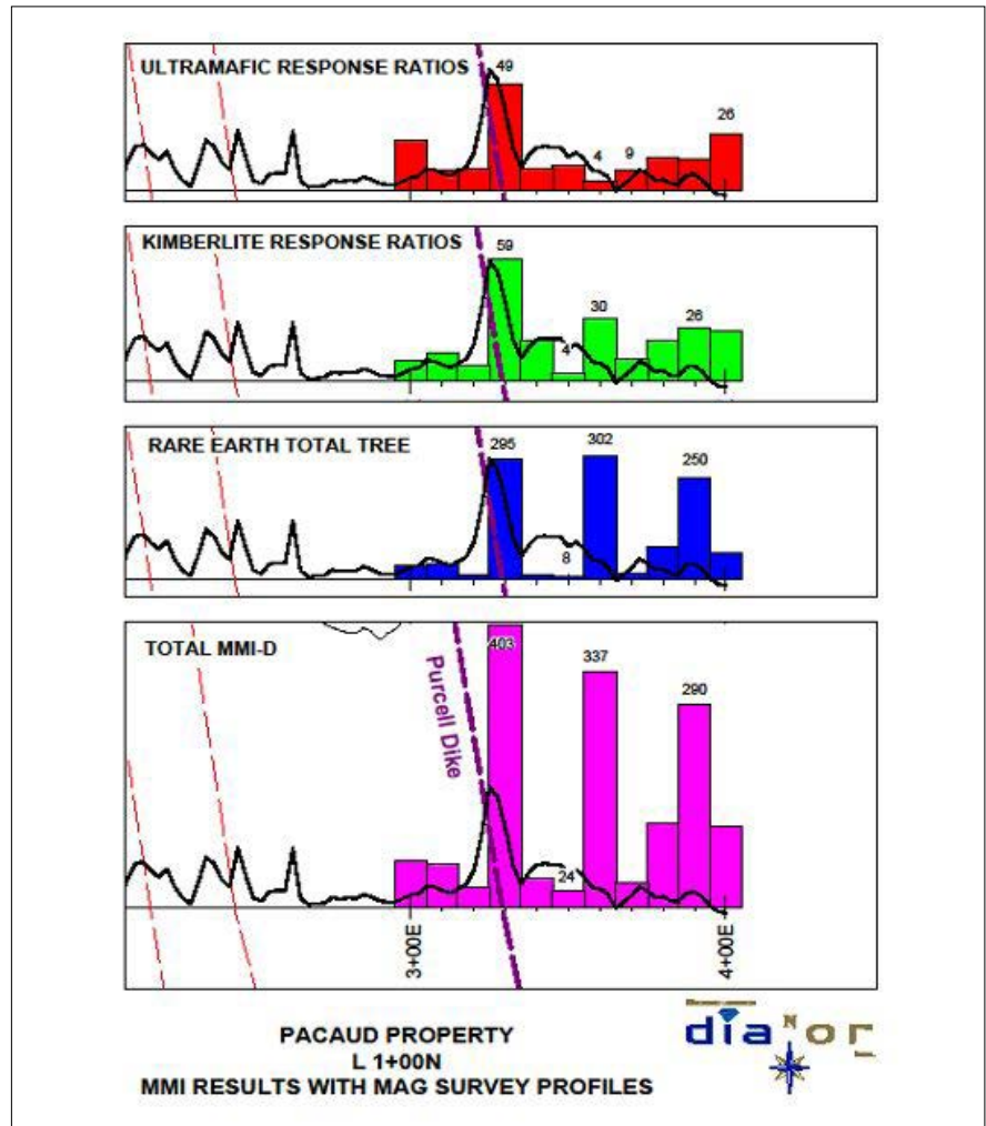
Figure 2: MMI™ Results Over the Purcell Dyke Set in Pacaud Township, Ontario
