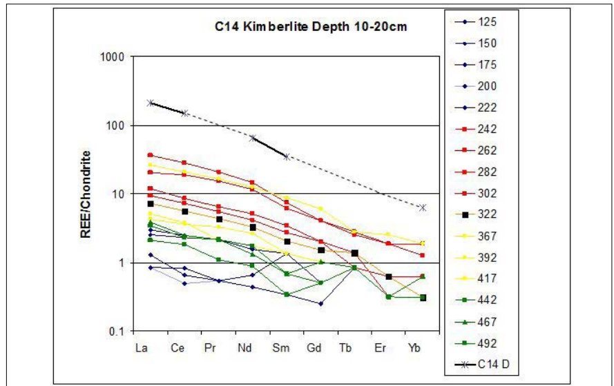
Figure 3: REE/Chondrite Plot for the C14 MMI™ data. C14D is from the Diatreme Facies of the C14 Pipe (McClenghan, 1999). Where the HREE Data are below Detection a Value of Half the Detection Limit is Used
