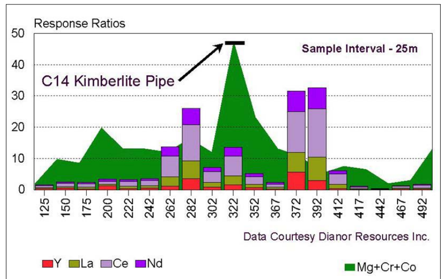
Figure 1: MMI™ Response Ratios (Ratio of Element to the Lowest Quartile Background Data) for the C14 Kimberlite for Selected Elements Sampled at 10-20cm Depth
